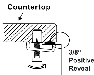
3/8" Positive Reveal
