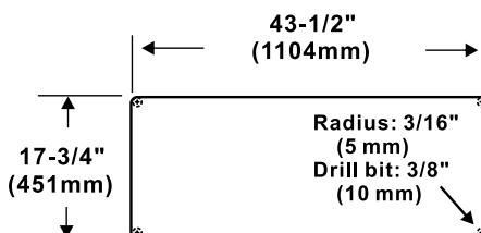
3/8" Positive Reveal
