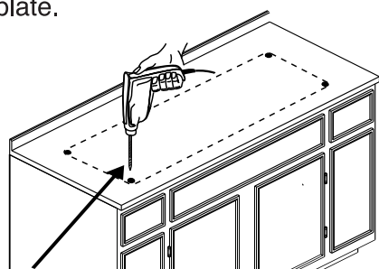
3/8" (10mm) diameter drill bit
