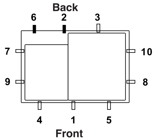
Distribution of topmount clips Clip tightening sequence
